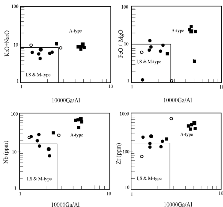
Fig. 6. K_2O + Na_2O , Nb, and Zr vs. 10000Ga/Al discrimination diagrams of [23]. Symbols as in Fig. 5.
