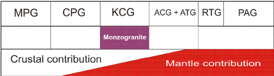
Figure 4. Monzogranite plot in the field of KCG (K-rich calc-alkaline granitoids [24].
