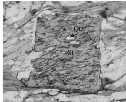
Fig. 7 Staurolite (St) porphyroblast containing a continuous curved trail of quartz (Qtz) inclusions. Width of photo corresponds to 0.8 mm. Sample 9, kyanite-bearing andalusite zone.
