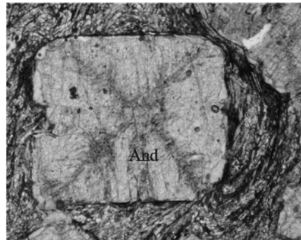
Fig. 10 Texturally sector-zone andalusite (And). Note well developed cleavage dome in right hand side of andalusite. Width of photo corresponds to 2.2 mm. Sample 55, kyanite-free andalusite zone.
