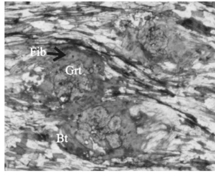
Fig. 12 Pseudomorphs after regional garnet altered mainly to fibrolite (after biotite). New crystals of thermal garnet are found growing in clusters. Width of photo corresponds to 2.2 mm. Sample 73, sillimanite zone.
