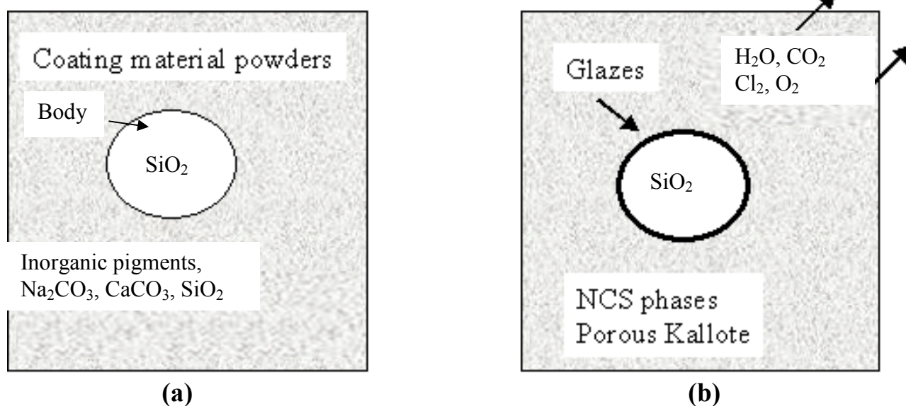
Fig. 1. Schematic procedures of the experimental setup of the cementation and calcination processes for the preparation of traditional ceramic glazes; (a) Before sintering, the system consist of ceramic support of quartz and coating powders of NCS and inorganic pigments; (b) After calcinations and sintering formation of glazes and the porous solid solution of amorphous NCS and Kallote.
