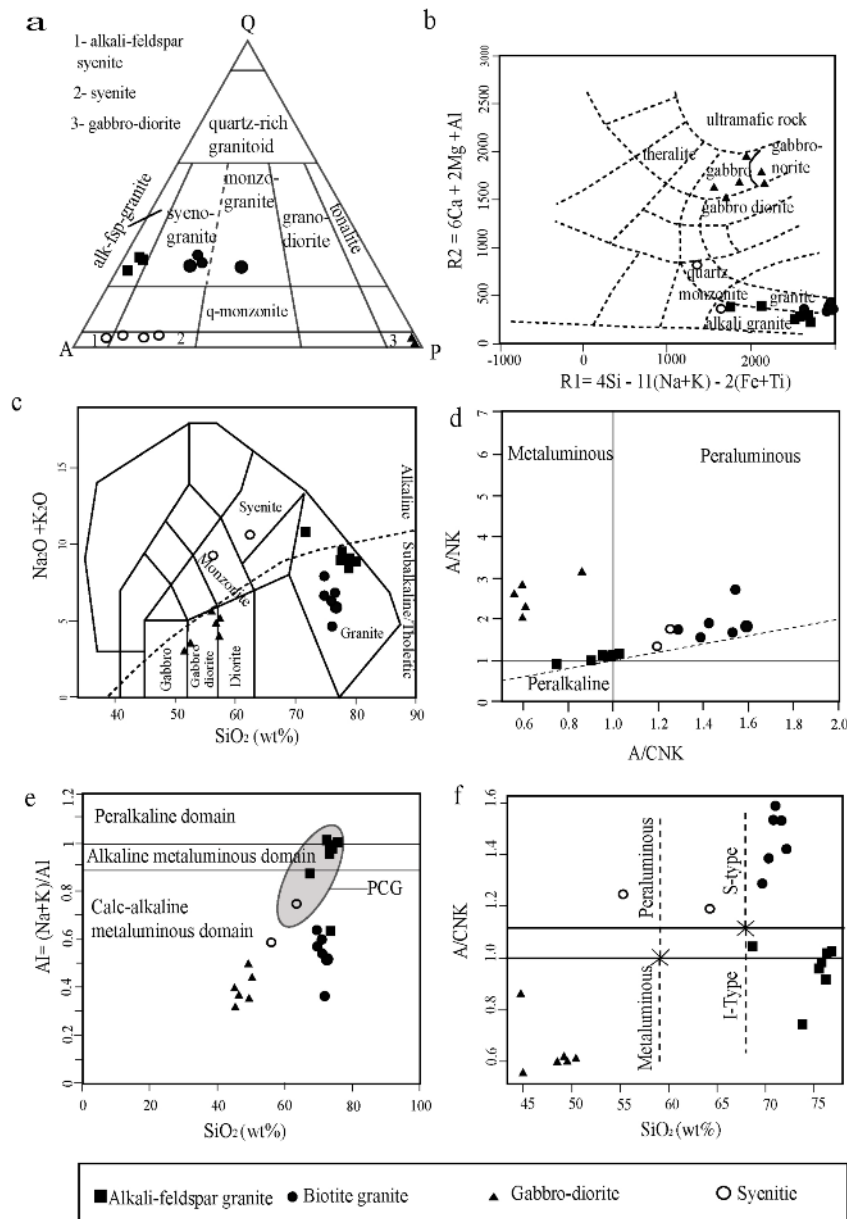
Fig. 5. Modal and chemical classification diagrams. (a) Modal classification of igneous rocks from [50] (b) R1-R2 cationic classification of [19]. (c) \text{Na}_2\text{O}+\text{K}_2\text{O} vs. \text{SiO}_2 from [20]. (d) \text{Al}/(\text{Na}+\text{K}) vs. \text{Al}/(\text{Ca}+\text{Na}+\text{K}) (mol. %): field boundaries are from [51]. (e) Alpaite index (AI) vs. \text{SiO}_2 diagram [52]. The post-collision granite (PCG) field is from [22]. (f) \text{SiO}_2 vs. \text{A}/\text{CNK} diagram. Peraluminous and metaluminous fields are after [53] and I-type and S-type fields are after [54].
