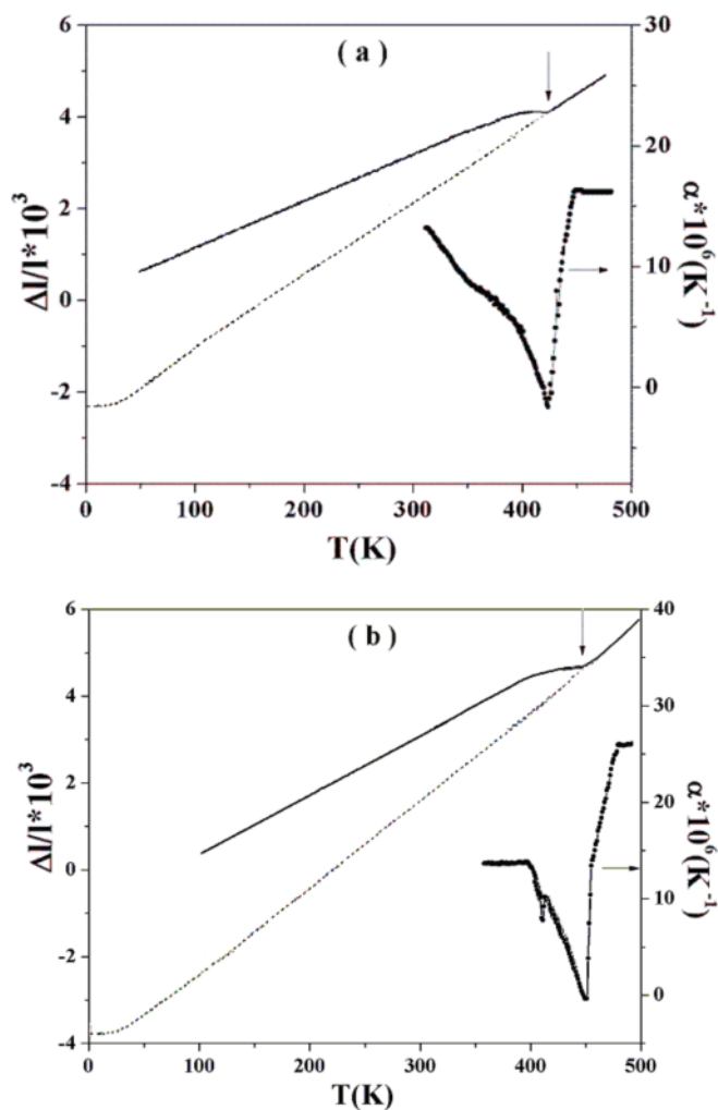
Fig. 4 Experimental thermal expansion \Delta l/l(T) and linear thermal expansion coefficient \alpha(T) curve of of \text{Nd}_6\text{Fe}_{13-x}\text{Co}_x\text{Cu} (a) x = 0 and (b) x = 1 samples. The dash line exhibits calculated lattice contribution to the thermal expansion. The arrows indicate the Néel temperature.
