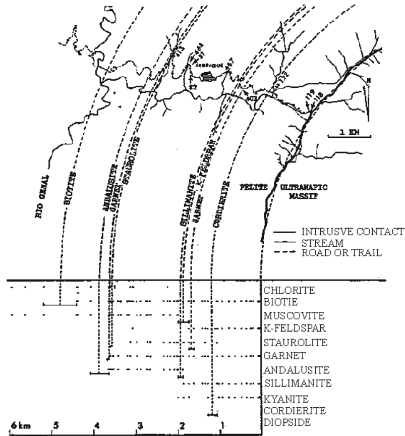
Fig. 3 Map of the Jubrigne sample traverse, north-west part of the Ronda aureole "Gneiss Series", Spain. (From Loomis, 1972, Fig.2).
