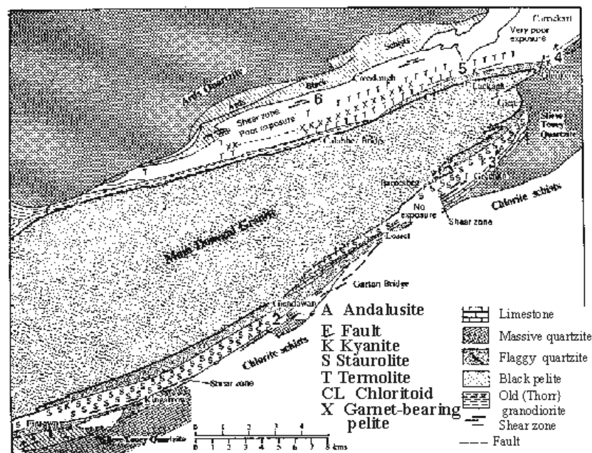
Fig. 2 Sample localities within the aureole of the Main Donegal granite. 1. Fintown, 2. Glenaboghill, 3. Loch Reelan, 4. Glenkeo, 5. Lachagh Bridge, 6. Owennagreeve river. (From Naggar and Atherton, 1970, Fig. 4).
