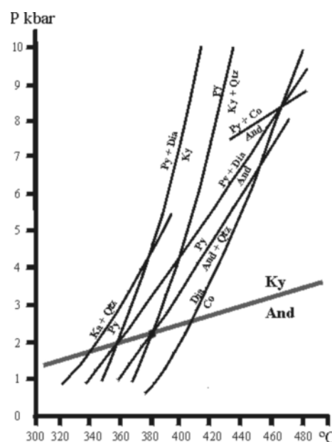
Fig. 9 Phase equilibrium diagram for the system \text{Al}_2\text{O}_3\text{-SiO}_2\text{-H}_2\text{O} . The invariant point (filled circle) formed by the intersection of the pyrophyllite = \text{Al}_2\text{SiO}_5 + quartz + water equilibrium with the kyanite = andalusite equilibrium indicates the lowest pressure for kyanite + quartz in a system with a\text{H}_2\text{O} = 1.0 . (From Holdaway, 1971).
