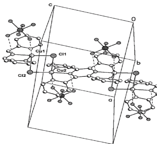
Figure 2 Cell drawing of the complex, [\{\text{CuCl}\}_2(\mu - \text{tpz})](\text{PF}_6)_2 . Selected bond lengths (Å) and bond angles (deg): Cu2-Cl2, 2.2431(12); Cu1-Cl2, 2.7196(13); Cu1-Cl2-Cu2, 83.20(4); Cl1-Cu1-Cl2, 96.80(4).
