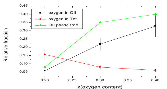
Fig 4 The relative OII phase fraction vs. x at 300 °C (error bars included).
