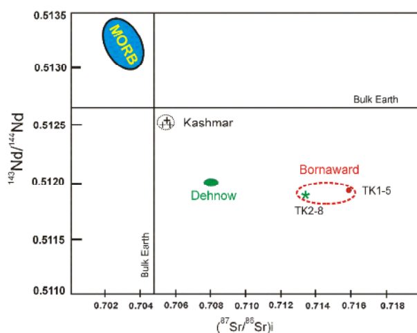
Figure 16. Plot of Initial ^{87}\text{Sr}/^{86}\text{Sr} versus Initial ^{143}\text{Nd}/^{144}\text{Nd} isotope values for Bornaward, Dehnow and Kashmar granitoid rocks.
