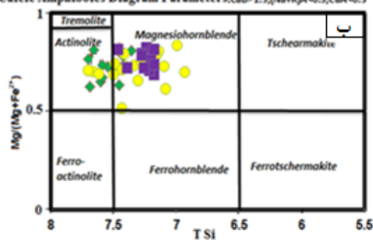
Calcic Amphiboles Diagram Parameters: Ca/B&gt;1.5; [Na+K]/A&lt;0.5; Ca/A&lt;0.5
