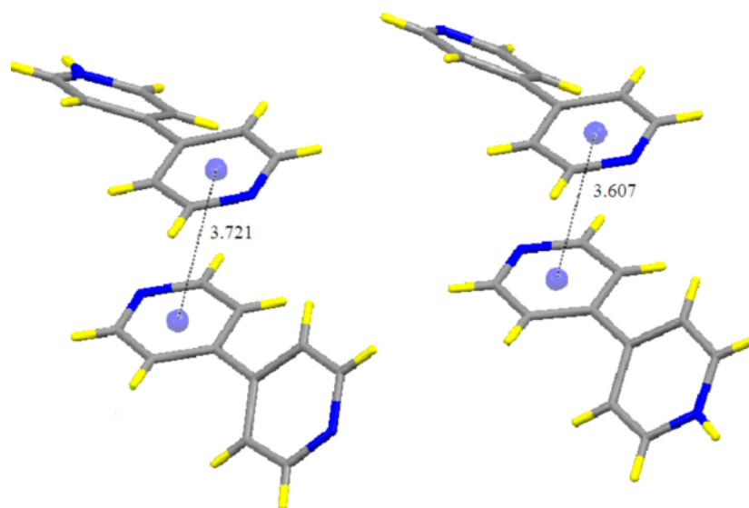
Fig. 3 \pi - \pi stacking interactions between aromatic rings of 4,4'-bipy and (4,4'-bipyH) + fragments with distances 3.6065(8) and 3.7216(8) Å for Cg4 \cdots Cg5 (1/2-x, -1/2 + y, 3/2-z) and (1/2-x, 1/2+y, 3/2-z) [Cg4 and Cg5 are the centroids for N3/C15-C17,C23,C24 and N5/C25-C27,C33,C34 rings, respectively].
